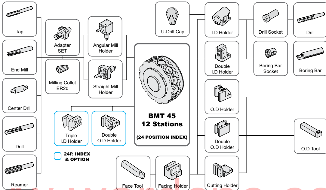
Mill Turret Tooling Parts Detail (SE2200MA/LMA/M/LM/LMC/LMSA/LMS/LMSC)
